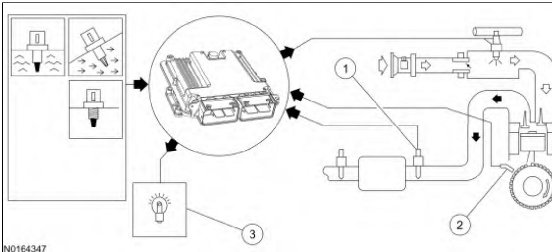
Air Fuel Ratio Imbalance Monitor
